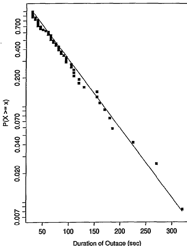
Fig. 4. Distribution of long \mathcal{D}_1 outages.
