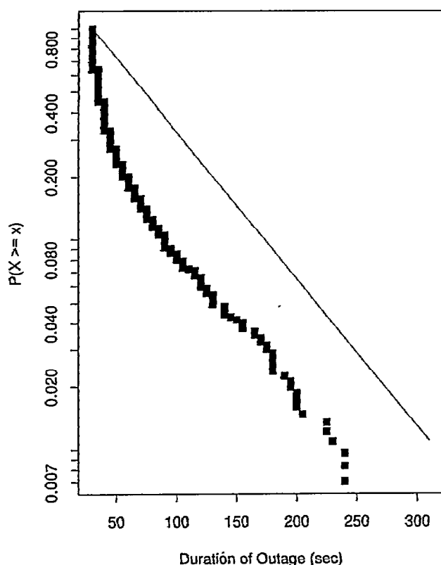
Fig. 5. Distribution of long D_2 outages.
