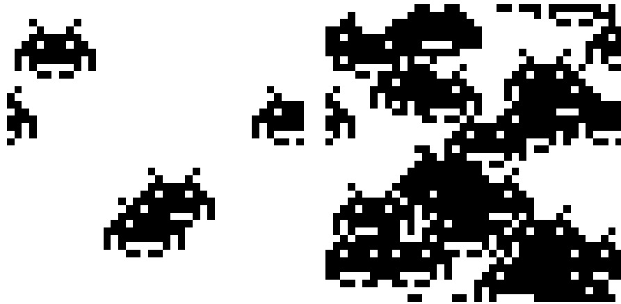
Figure E.1: Filling a screen with Space Invaders. The left-hand image places four copies of a 46-pixel sprite in random positions on a 40 \times 40 screen. The right-hand image does the same thing with 24 copies.
